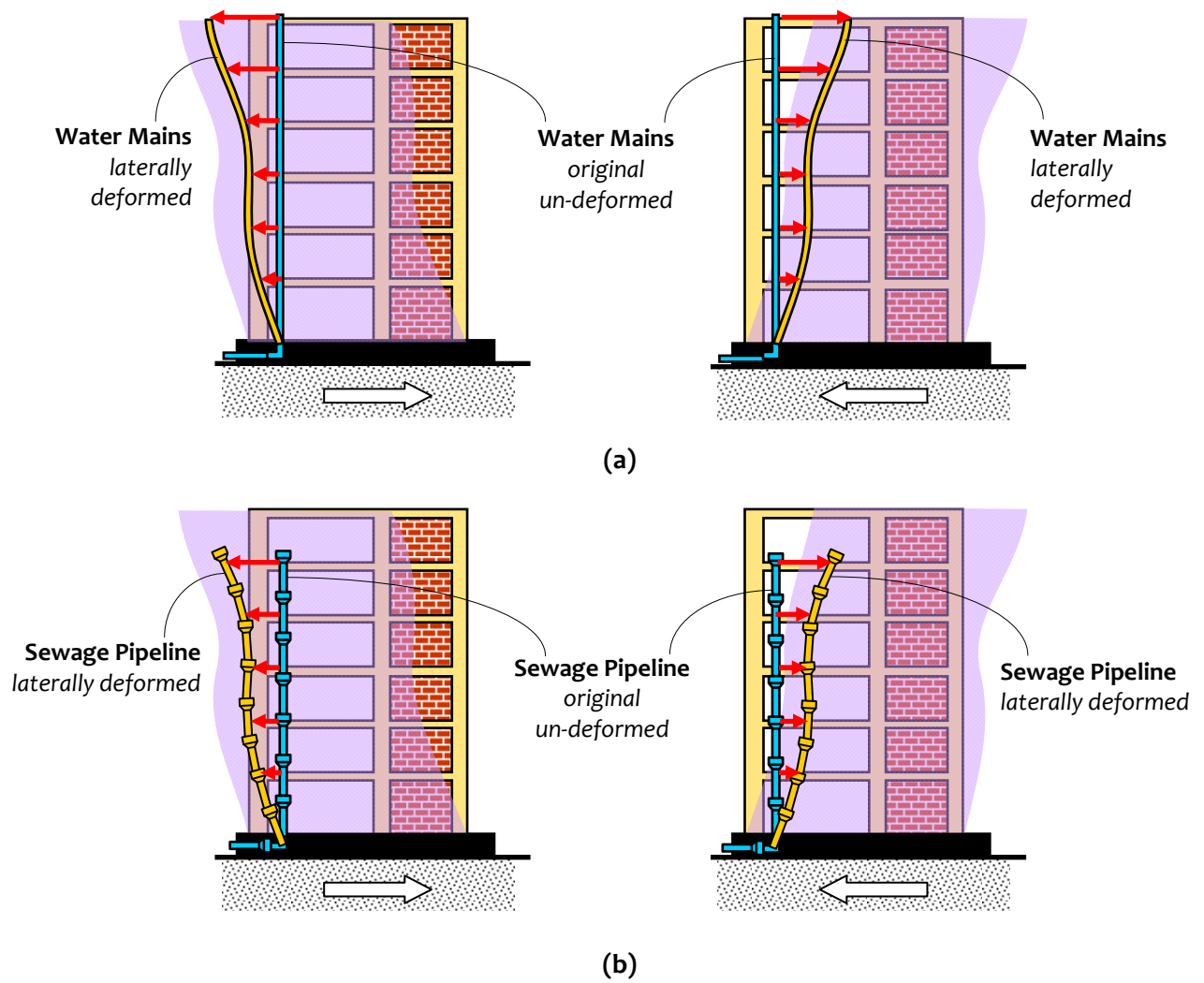
Figure 3.23: Inter-storey Relative Displacement: Linear NSEs need to sustain lateral translational strains without failure: (a) Water pipelines, and (b) Sewage pipes
