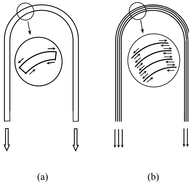
Fig. 2-6: Wrapping with (a) thick strips and (b) non-laminated straps.
