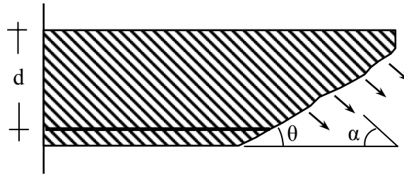
Fig. 5-5: Contribution of FRP to shear capacity.
