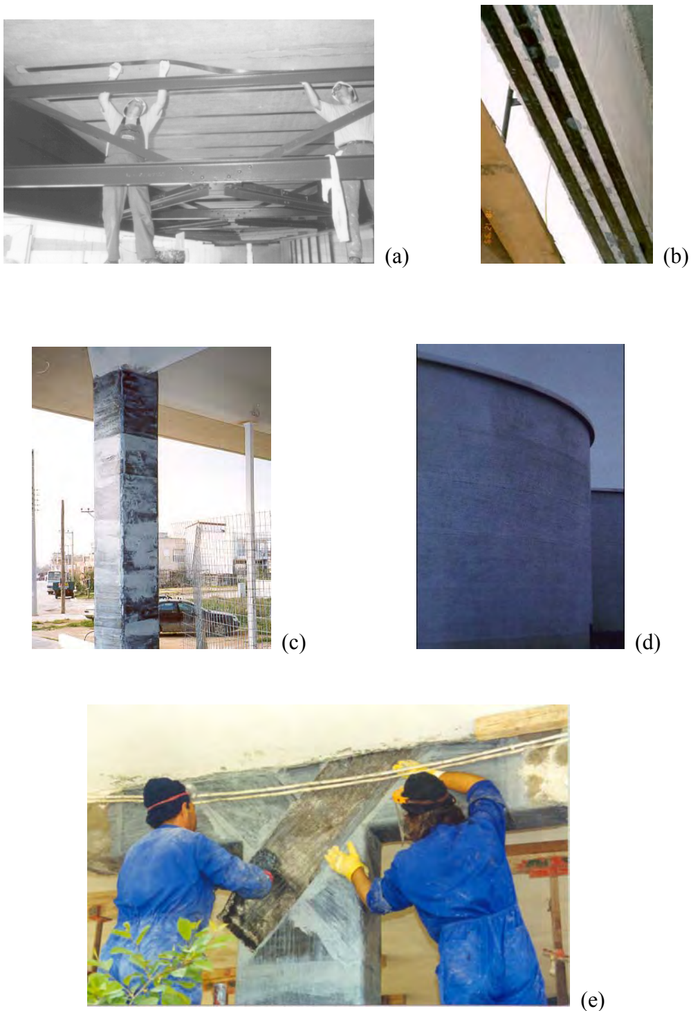
Fig. 1-2: Typical FRP applications as strengthening materials of RC structures: (a) flexural strengthening of slab; (b) flexural strengthening of beam; (c) shear strengthening and confinement of column; (d) wrapping of concrete tank; (e) shear strengthening of beam-column joint.
